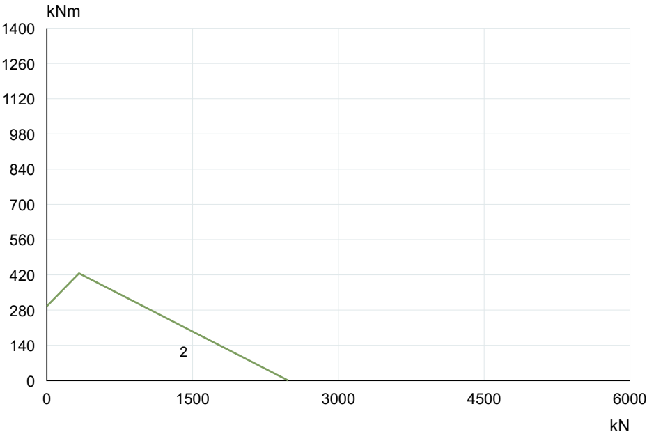
VI096A00 · Curva original 1S 2 · PDF p15
