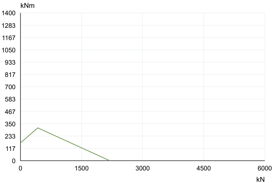
La Leonessa VI085A05 — Load capacity curve
