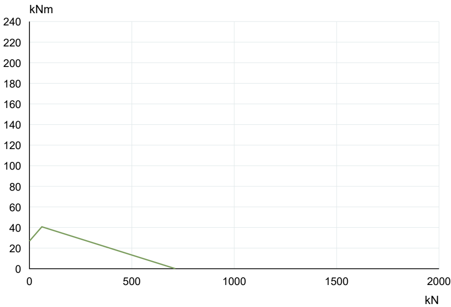
La Leonessa VI040A01 — Load capacity curve
