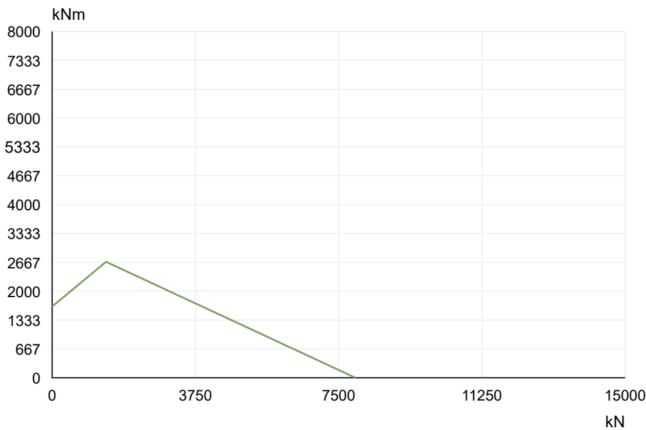
La Leonessa VE180A05 — Load capacity curve
