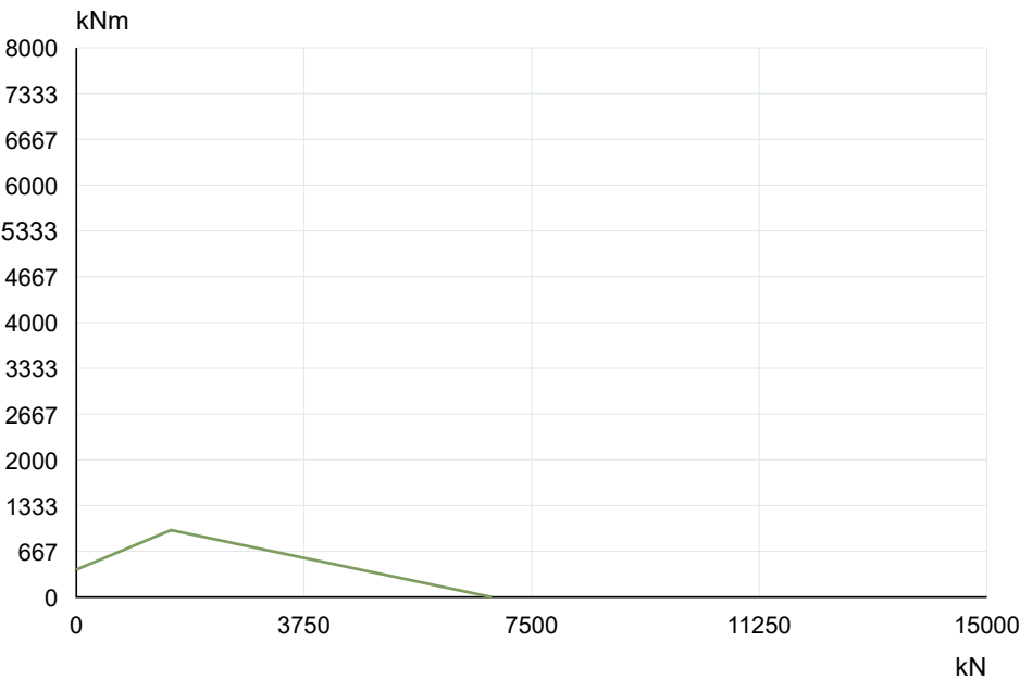
La Leonessa VE160A04 — Load capacity curve
