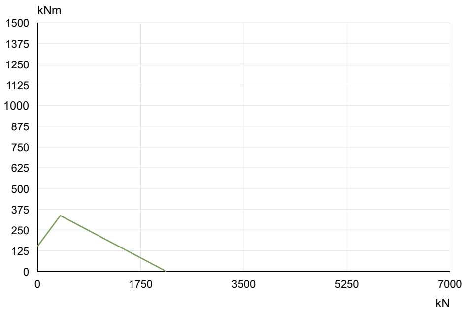
La Leonessa VE104A02 — Load capacity curve
