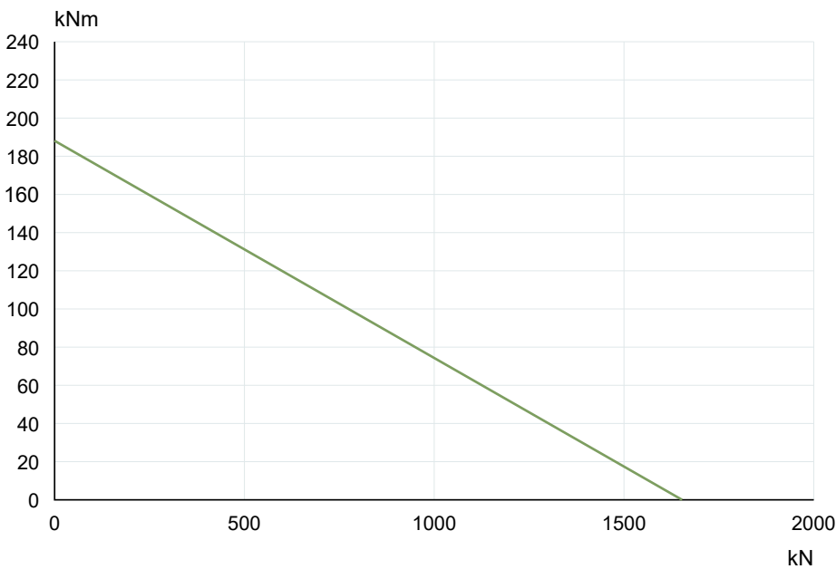
La Leonessa VE069A05 — Load capacity curve
