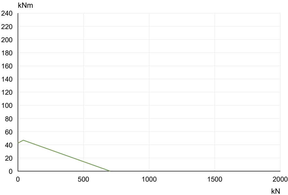
La Leonessa VE040A01 — Load capacity curve
